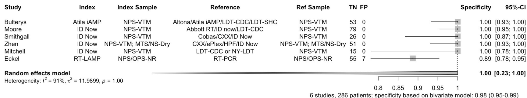
Figure s8d. Test accuracy studies evaluating rapid isothermal NAAT test vs. single standard non-rapid lab-based NAAT or composite reference standard when available, specificity analysis excluding studies that used different sample source and/or transport media in index sample compared to reference sample
