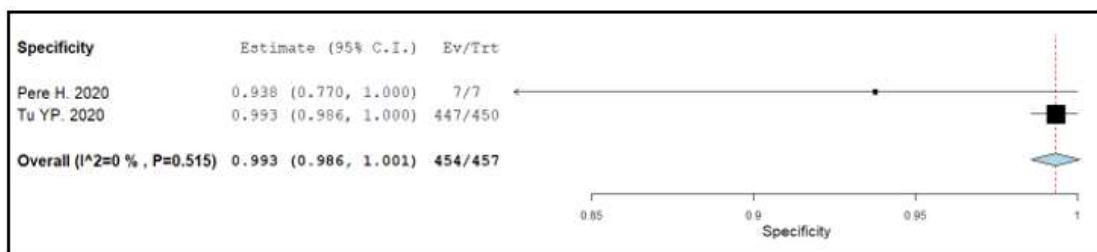
Figure s12. Specificity Pooled by Proportion from 2 studies that reported specificity
